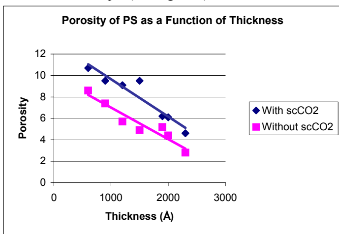
Figure 1. Porosity of PS, with and without scCO 2 , as a function of thickness
