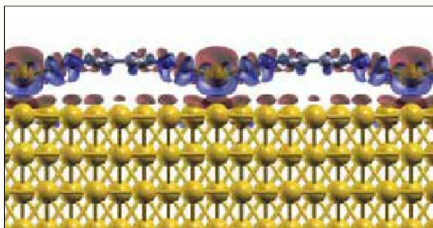
Computed electron density difference before and after aromatic isocyanide molecules adsorb on the surface of gold and form a one-dimensional chain bridged by surface atoms. The red represents electron gain and the blue electron loss.
